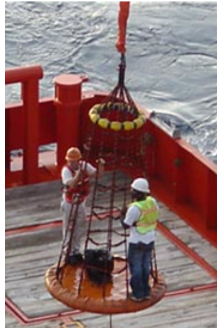
Personnel Transfer Nets Overall Length: 10m Floatation: Enough to float five (5) men
